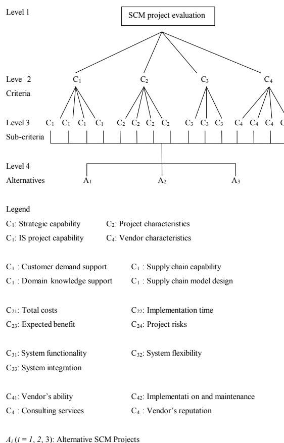
Figure 2 The hierarchical structure of the SCM project selection
