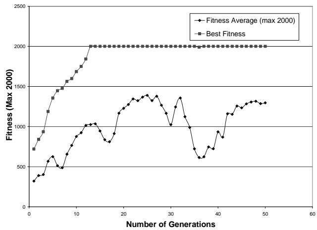
Fig. 13. Progression of average fitness of the population vs. number of Generations
