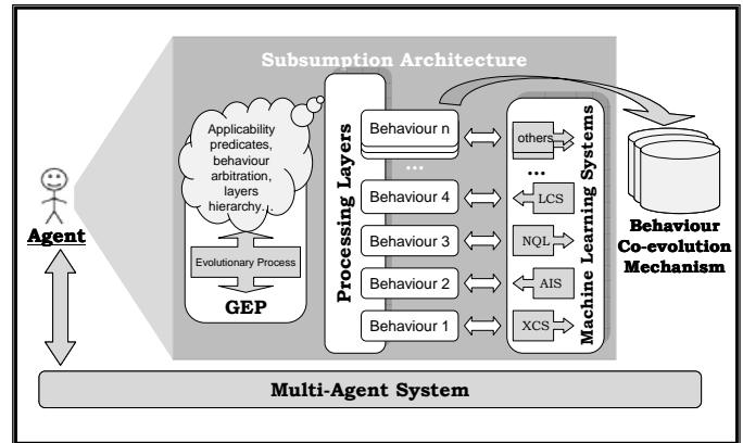
Fig. 5. Hybrid and Evolutionary Architecture for Cognitive Agents
