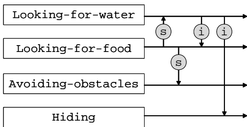
Fig. 16. Fragment Phenotype of an Initial Agent's Architecture
