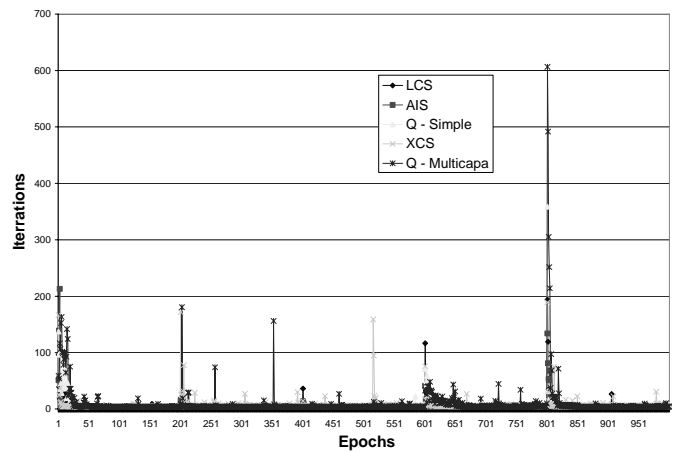
Figure 10. Learning Curve of each MLS
