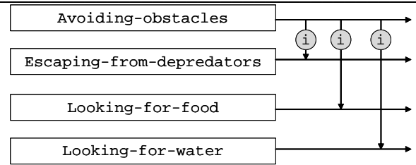
Fig. 18. Fragment Phenotype Agent's Architecture after 326 evolutionary generations
