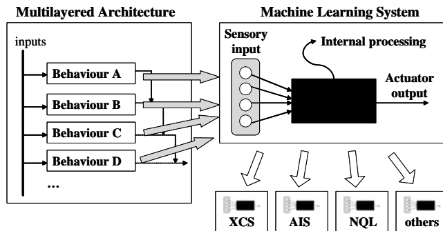
Fig. 6. Multilayered Architecture connecting with MLS interface
