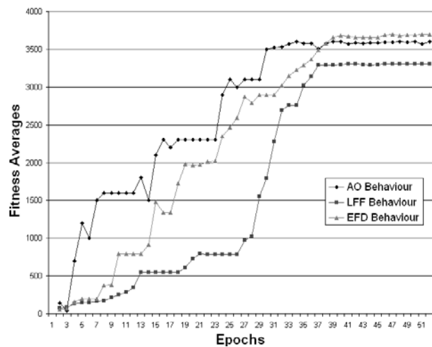
Fig. 11. Evolution convergence rate in 3 behaviour pools
