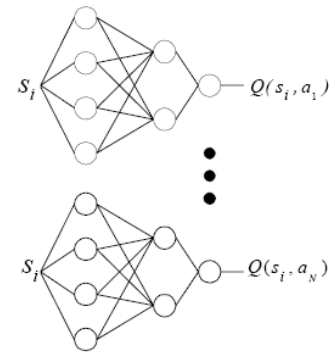
Fig. 4. Q-function approximation by a set of Neural Networks [11]
