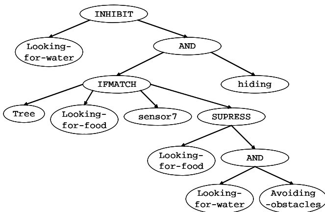
Fig. 15. Fragment Genotype of an initial Agent's Architecture
