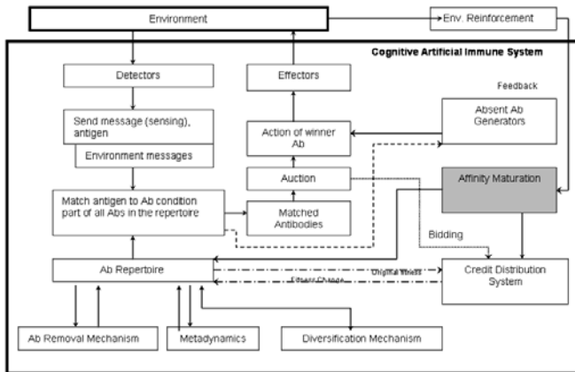
Fig. 3. Flow diagram of the proposed cognitive artificial immune system (ACIS) [9]
