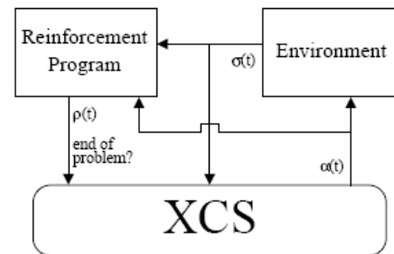
Fig. 2. XCS interacts with an Environment and a Reinforcement Program [5]
