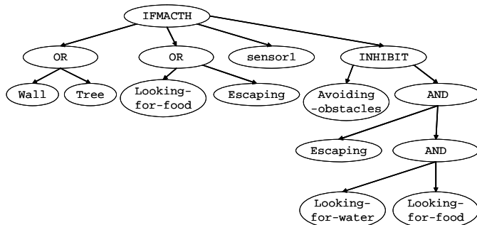
Fig. 17. Genotype Agent's Architecture after 326 evolutionary generations
